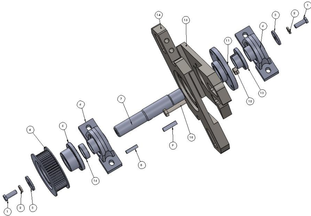
Quadwheel® Drive Assembly
